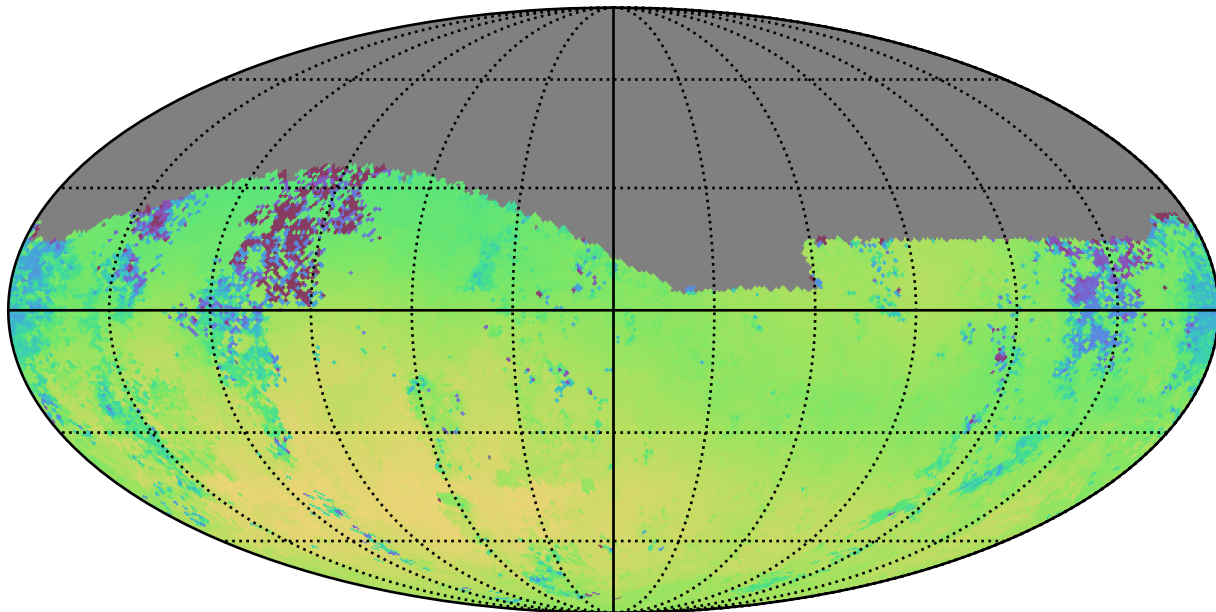
weather_cloudso14v3.4_10yrs Yr 1 g band: Median skyBrightness
