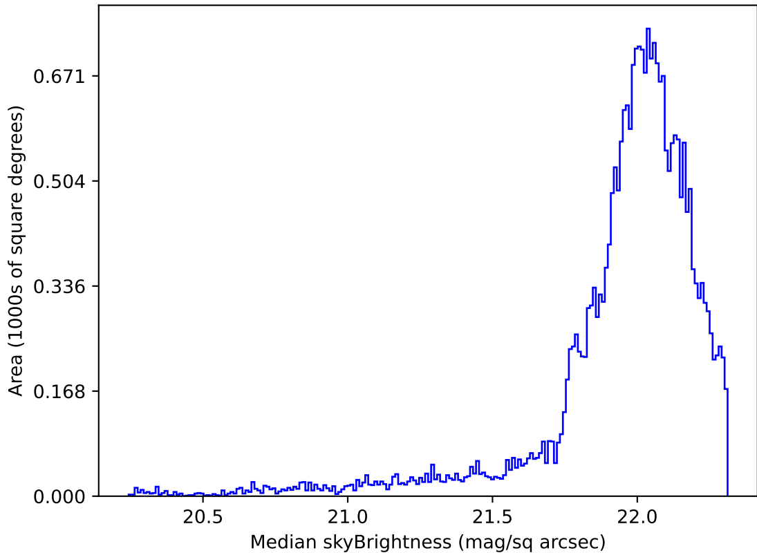
weather_cloudso14v3.4_10yrs Yr 1 g band: Median skyBrightness
