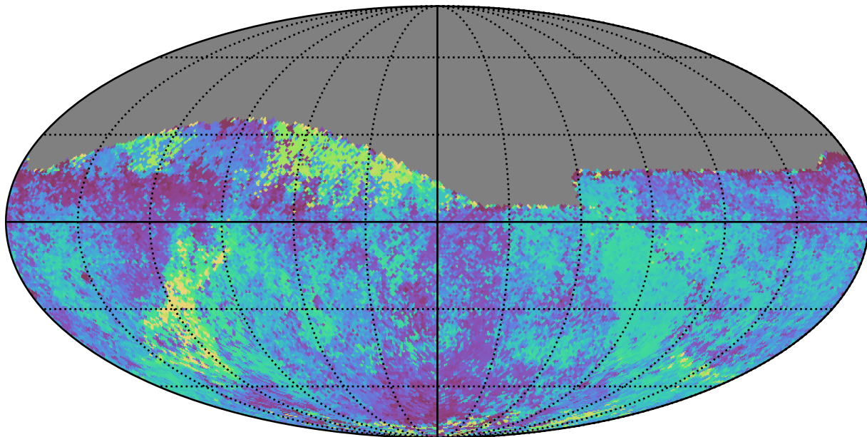
weather_cloudso14v3.4_10yrs Yr 1 all bands: Median skyBrightness
