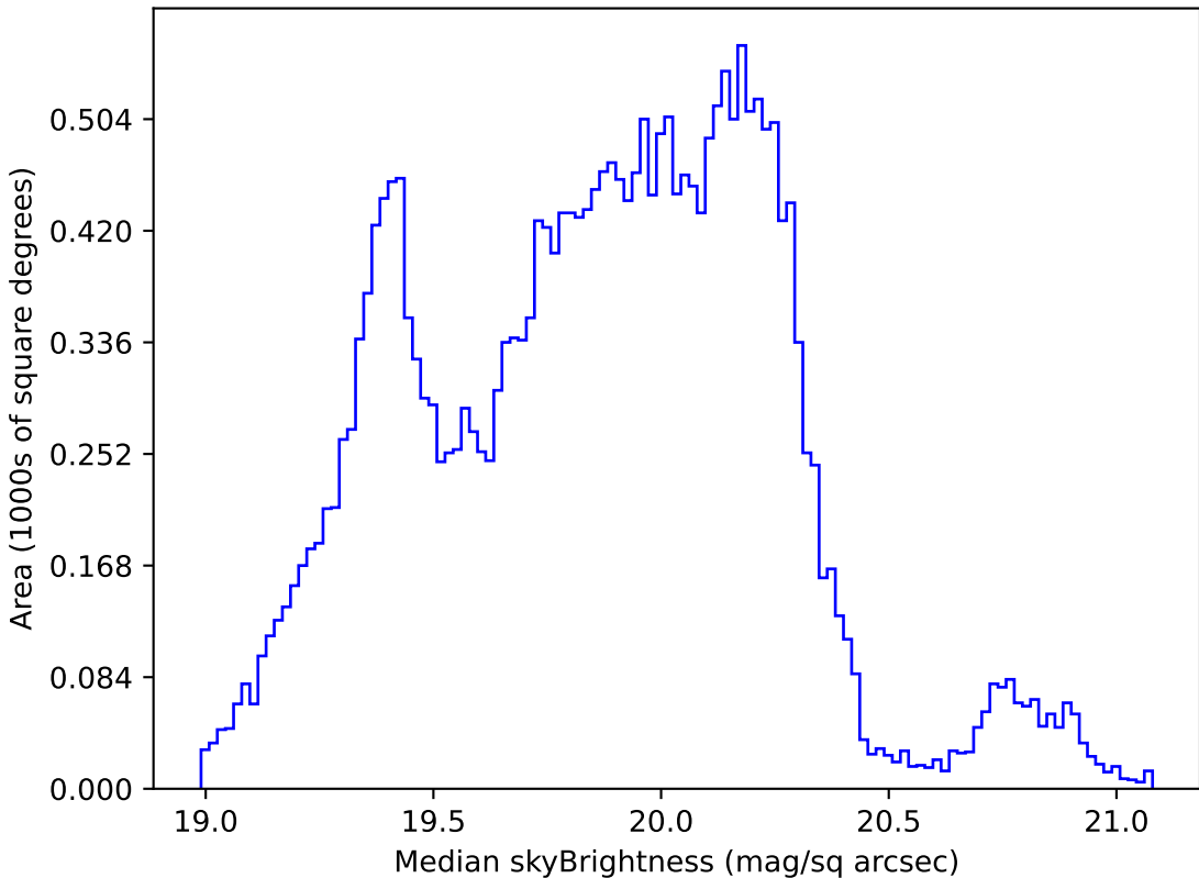
weather_cloudso14v3.4_10yrs Yr 1 all bands: Median skyBrightness
