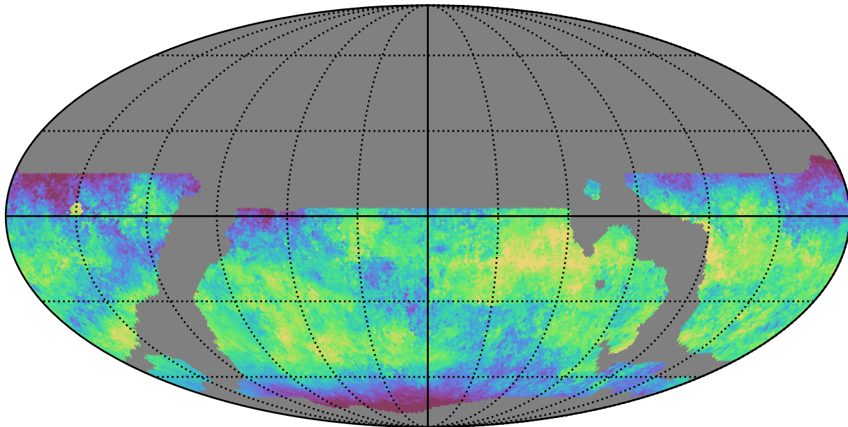
weather_cloudso14v3.4_10yrs WFD z band: Median skyBrightness
