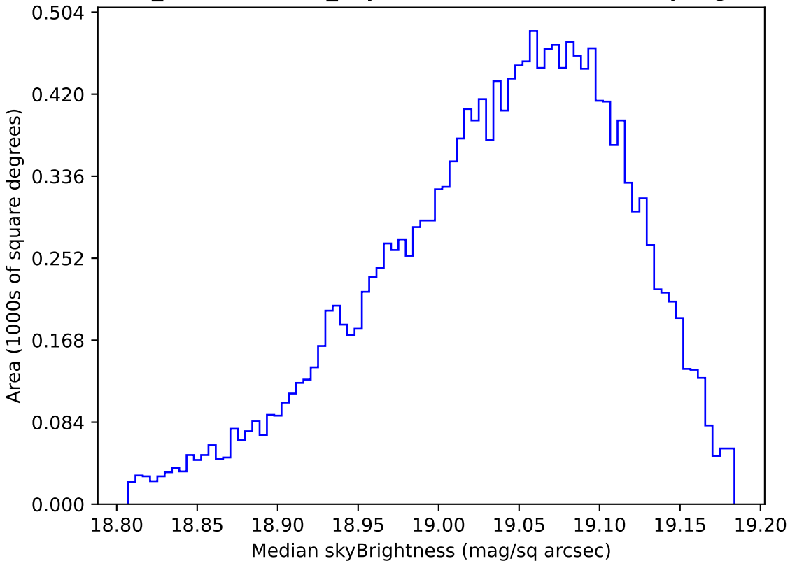
weather_cloudso14v3.4_10yrs WFD z band: Median skyBrightness
