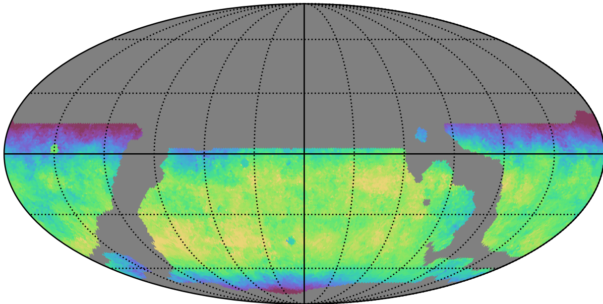
weather_cloudso14v3.4_10yrs WFD y band: Median skyBrightness
