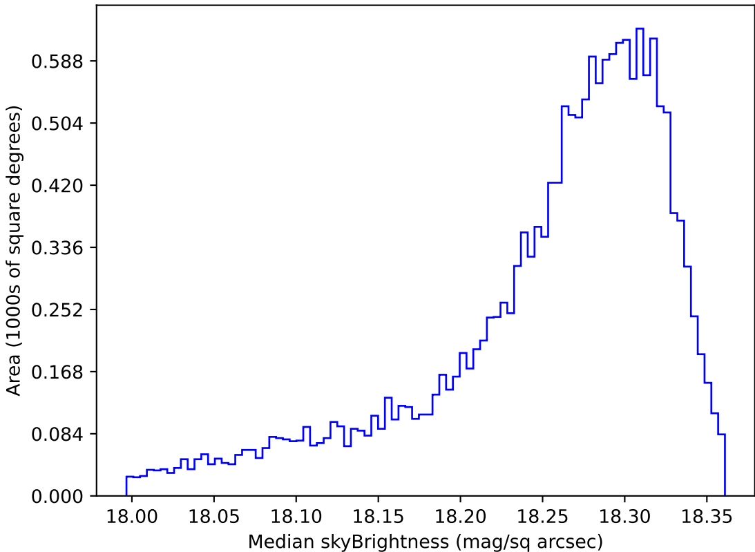
weather_cloudso14v3.4_10yrs WFD y band: Median skyBrightness
