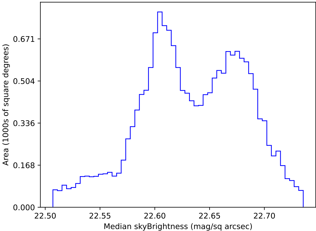
weather_cloudso14v3.4_10yrs WFD u band: Median skyBrightness
