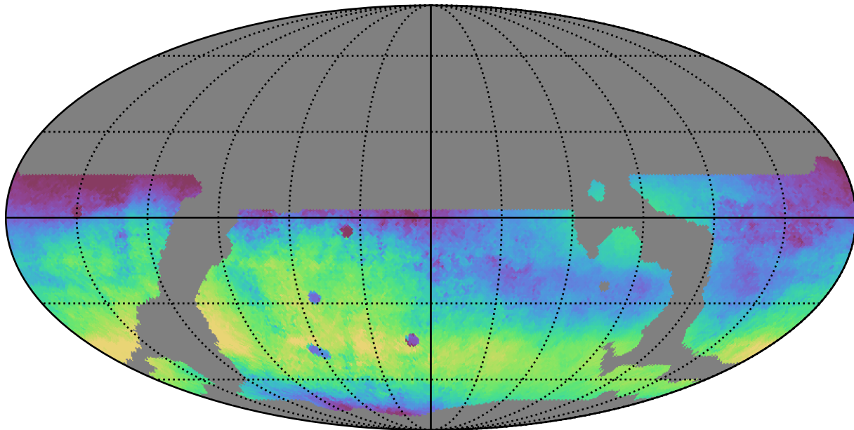
weather_cloudso14v3.4_10yrs WFD r band: Median skyBrightness
