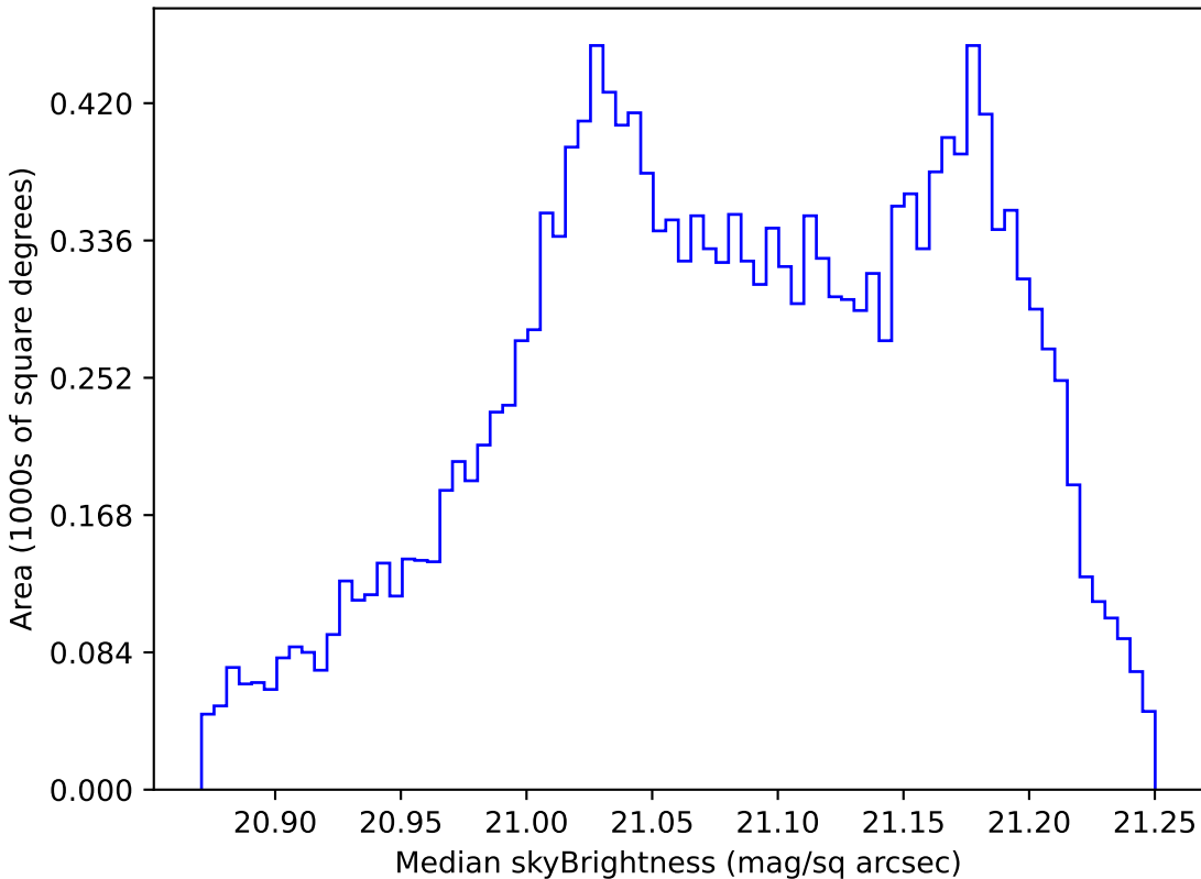
weather_cloudso14v3.4_10yrs WFD r band: Median skyBrightness
