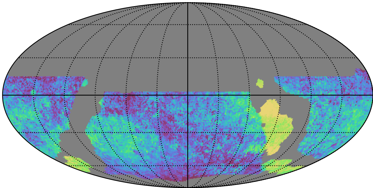
weather_cloudso14v3.4_10yrs WFD all bands: Median skyBrightness
