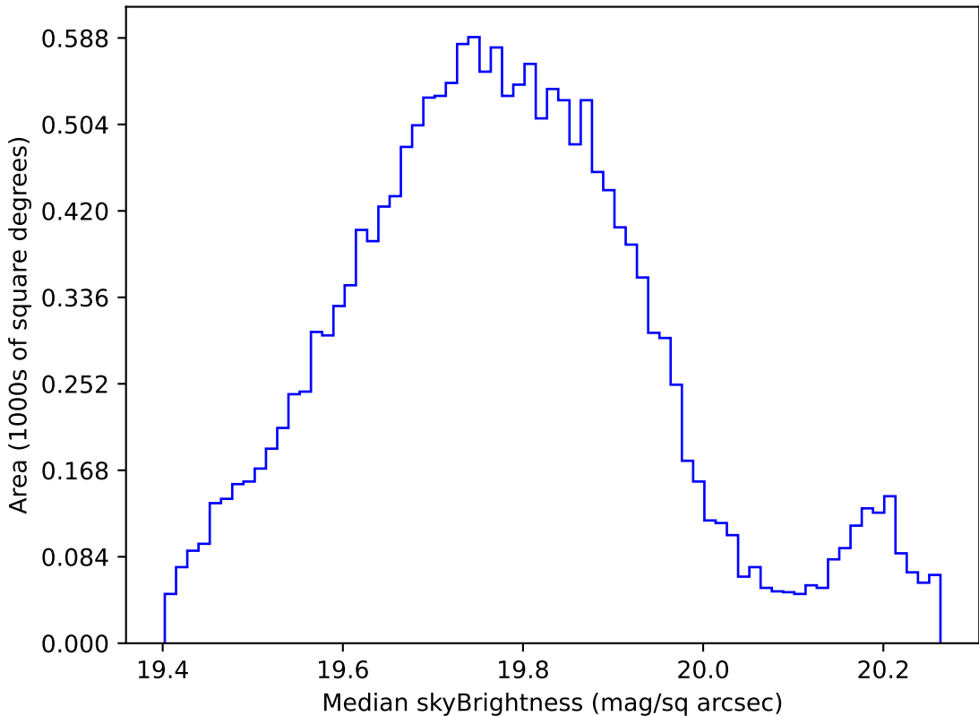
weather_cloudso14v3.4_10yrs WFD all bands: Median skyBrightness
