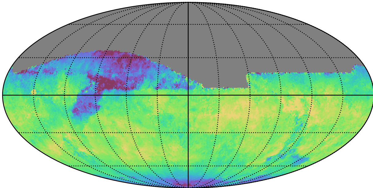
weather_cloudso14v3.4_10yrs All sky z band: Median skyBrightness
