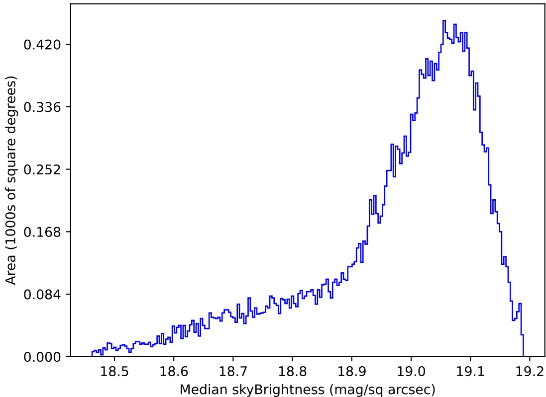
weather_cloudso14v3.4_10yrs All sky z band: Median skyBrightness
