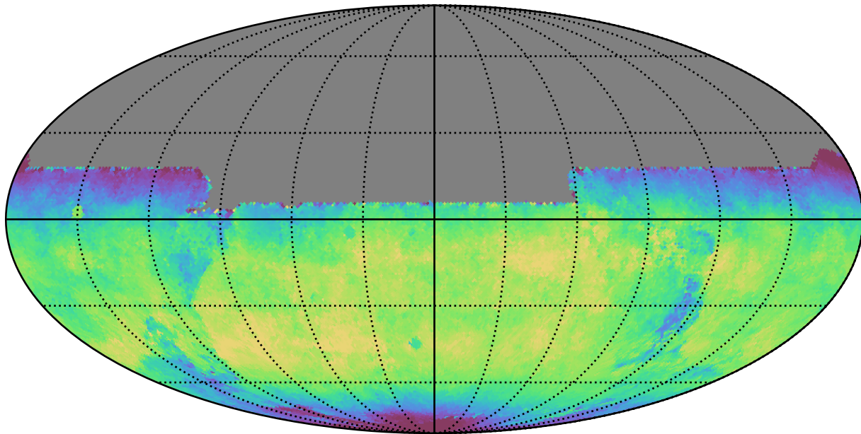
weather_cloudso14v3.4_10yrs All sky y band: Median skyBrightness
