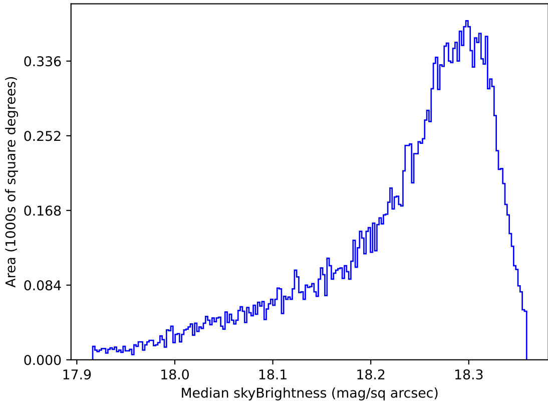
weather_cloudso14v3.4_10yrs All sky y band: Median skyBrightness
