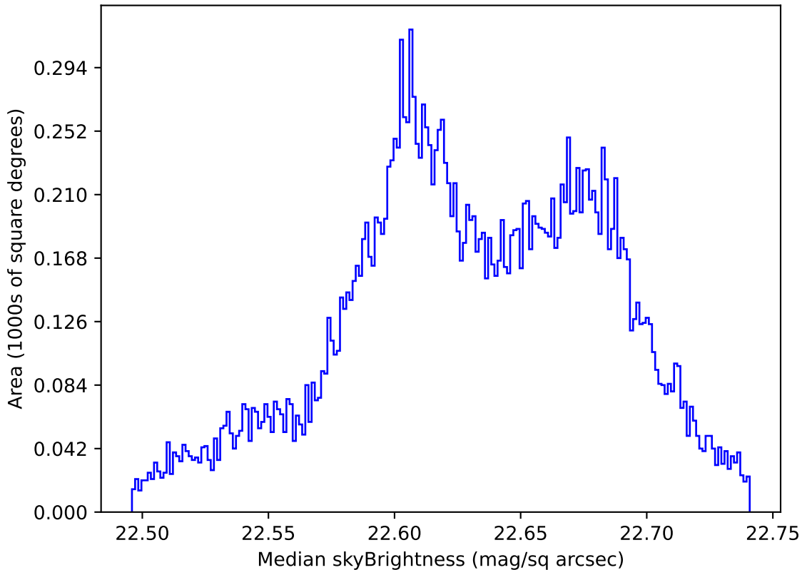
weather_cloudso14v3.4_10yrs All sky u band: Median skyBrightness
