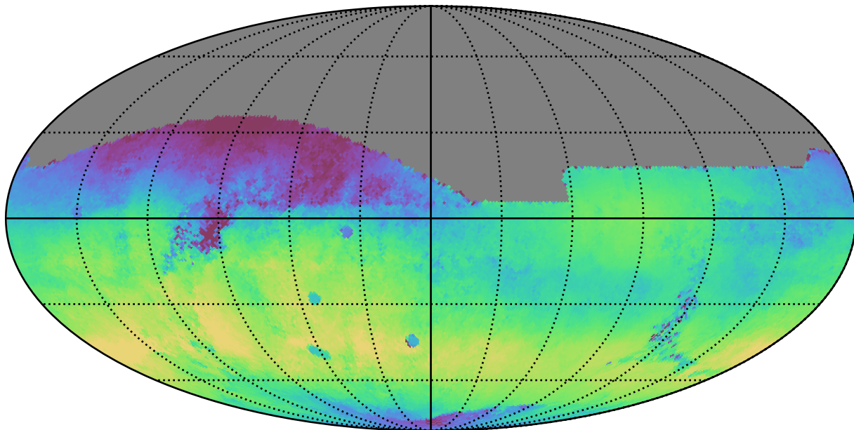
weather_cloudso14v3.4_10yrs All sky r band: Median skyBrightness
