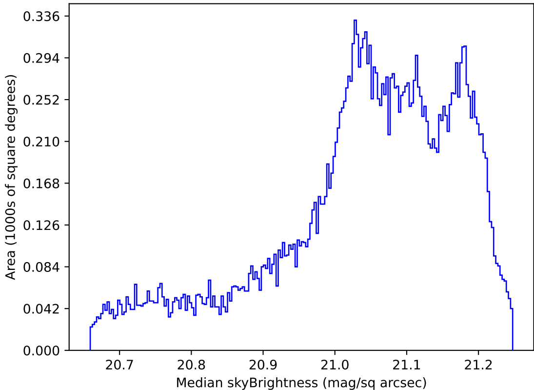
weather_cloudso14v3.4_10yrs All sky r band: Median skyBrightness
