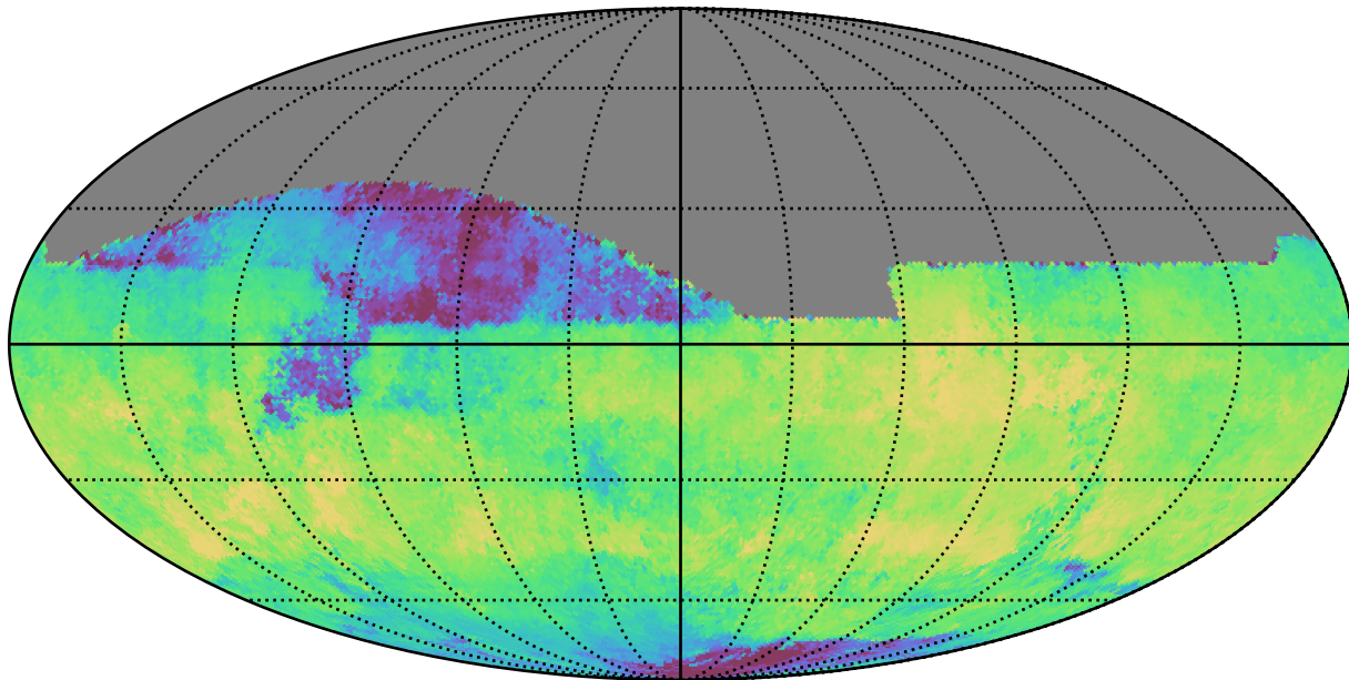
weather_cloudso14v3.4_10yrs All sky i band: Median skyBrightness
