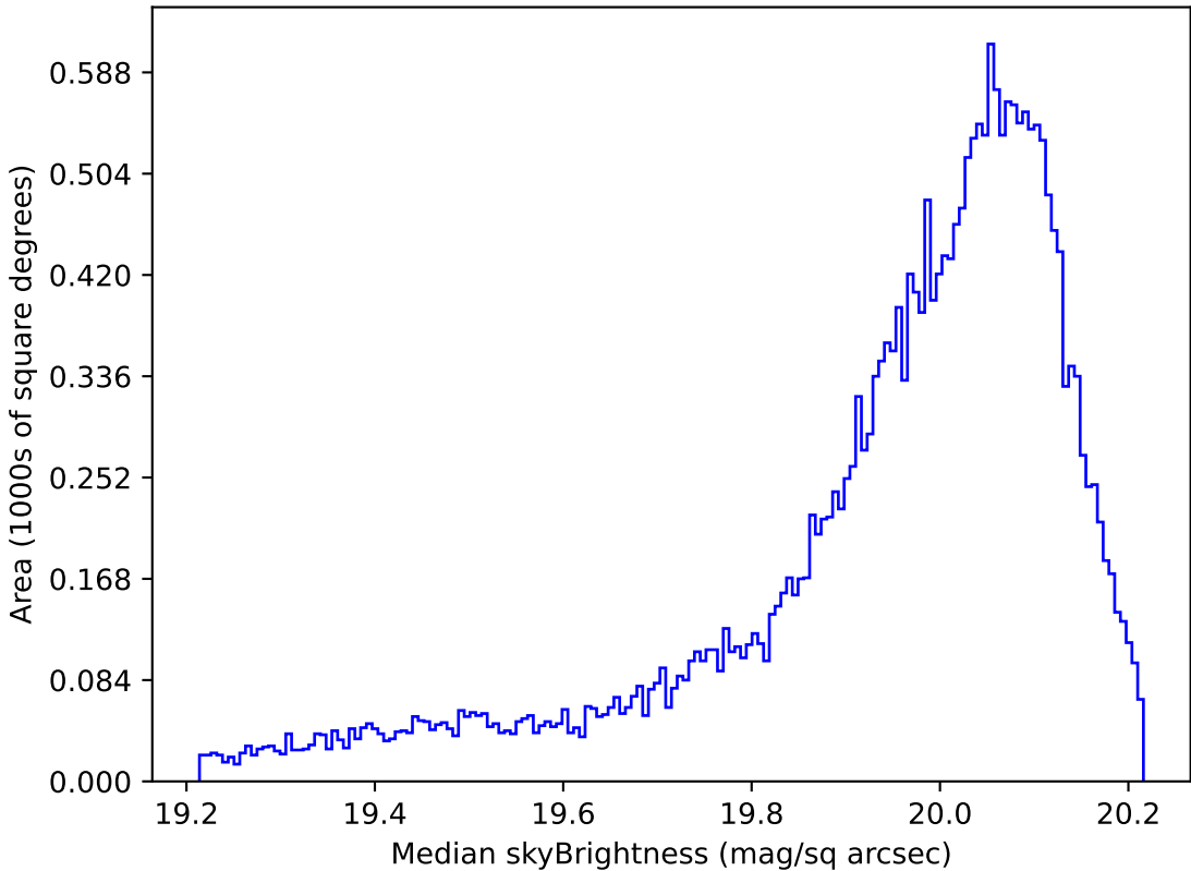
weather_cloudso14v3.4_10yrs All sky i band: Median skyBrightness
