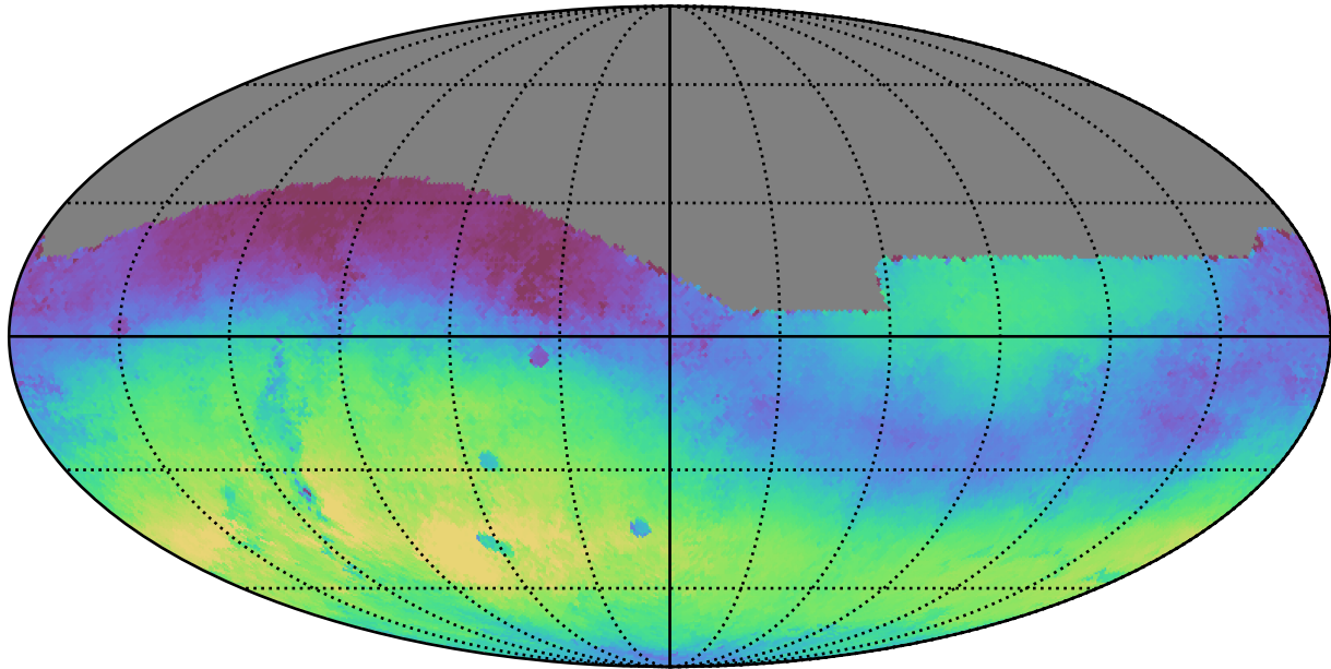
weather_cloudso14v3.4_10yrs All sky g band: Median skyBrightness
