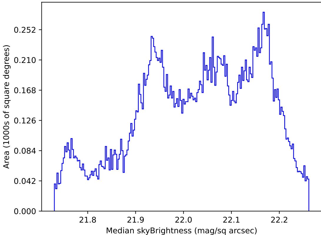
weather_cloudso14v3.4_10yrs All sky g band: Median skyBrightness
