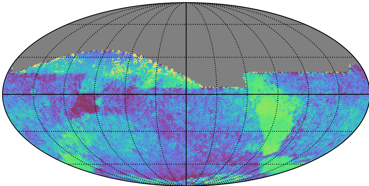
weather_cloudso14v3.4_10yrs All sky all bands: Median skyBrightness
