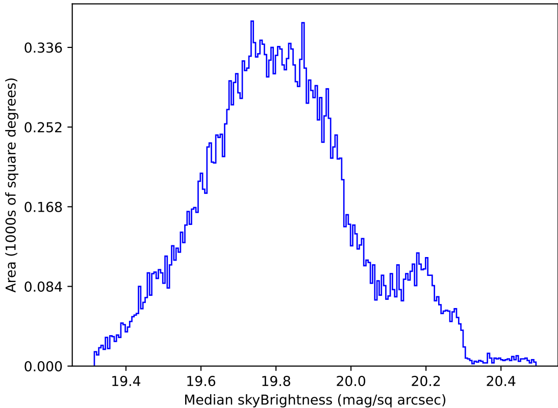
weather_cloudso14v3.4_10yrs All sky all bands: Median skyBrightness
