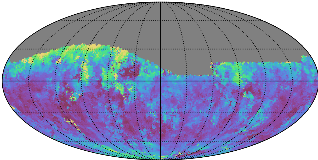
weather_cloudso14v3.4_10yrs Yr 1 z band: Median seeingGeom
