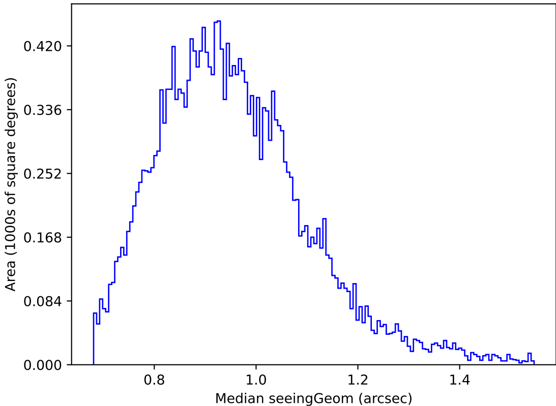
weather_cloudso14v3.4_10yrs Yr 1 u band: Median seeingGeom
