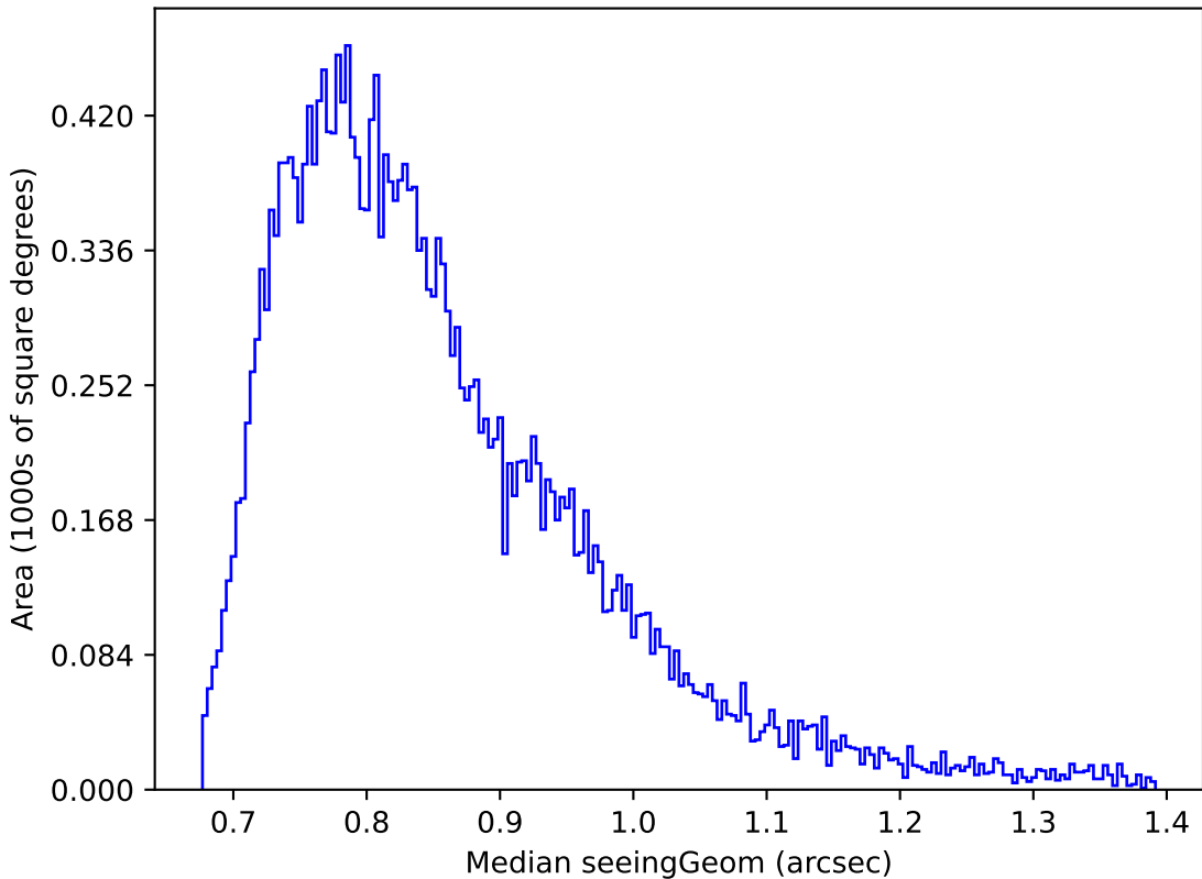
weather_cloudso14v3.4_10yrs Yr 1 i band: Median seeingGeom
