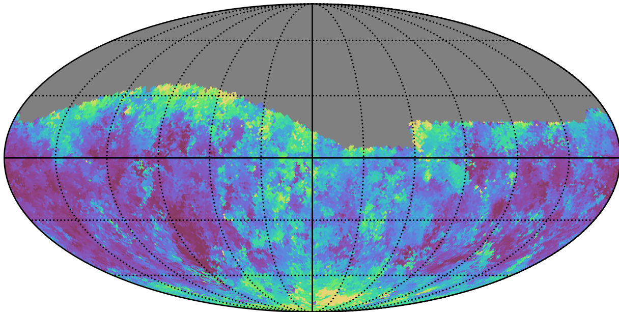
weather_cloudso14v3.4_10yrs Yr 1 g band: Median seeingGeom
