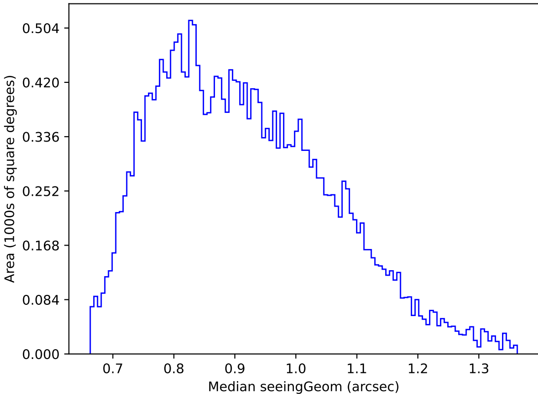
weather_cloudso14v3.4_10yrs Yr 1 g band: Median seeingGeom
