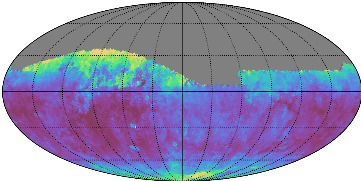
weather_cloudso14v3.4_10yrs Yr 1 all bands: Median seeingGeom
