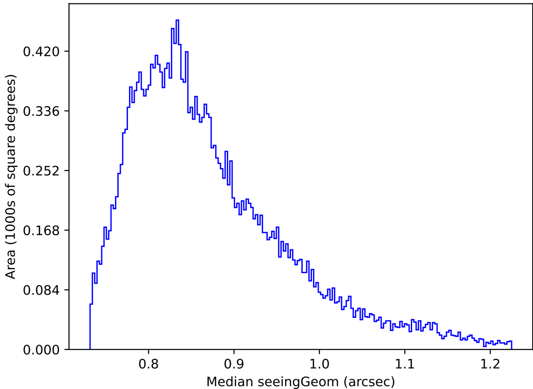
weather_cloudso14v3.4_10yrs Yr 1 all bands: Median seeingGeom
