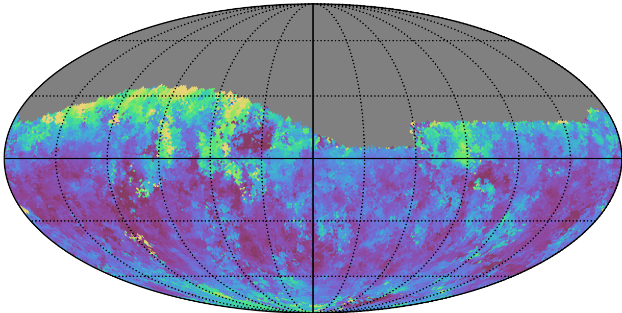
weather_cloudso14v3.4_10yrs Yr 1 z band: Median seeingEff
