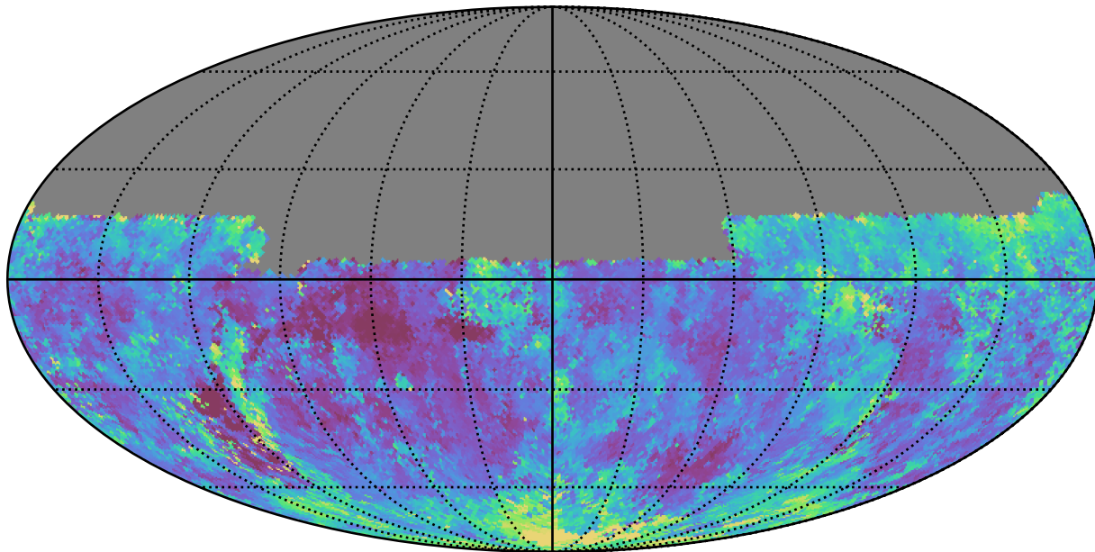
weather_cloudso14v3.4_10yrs Yr 1 y band: Median seeingEff
