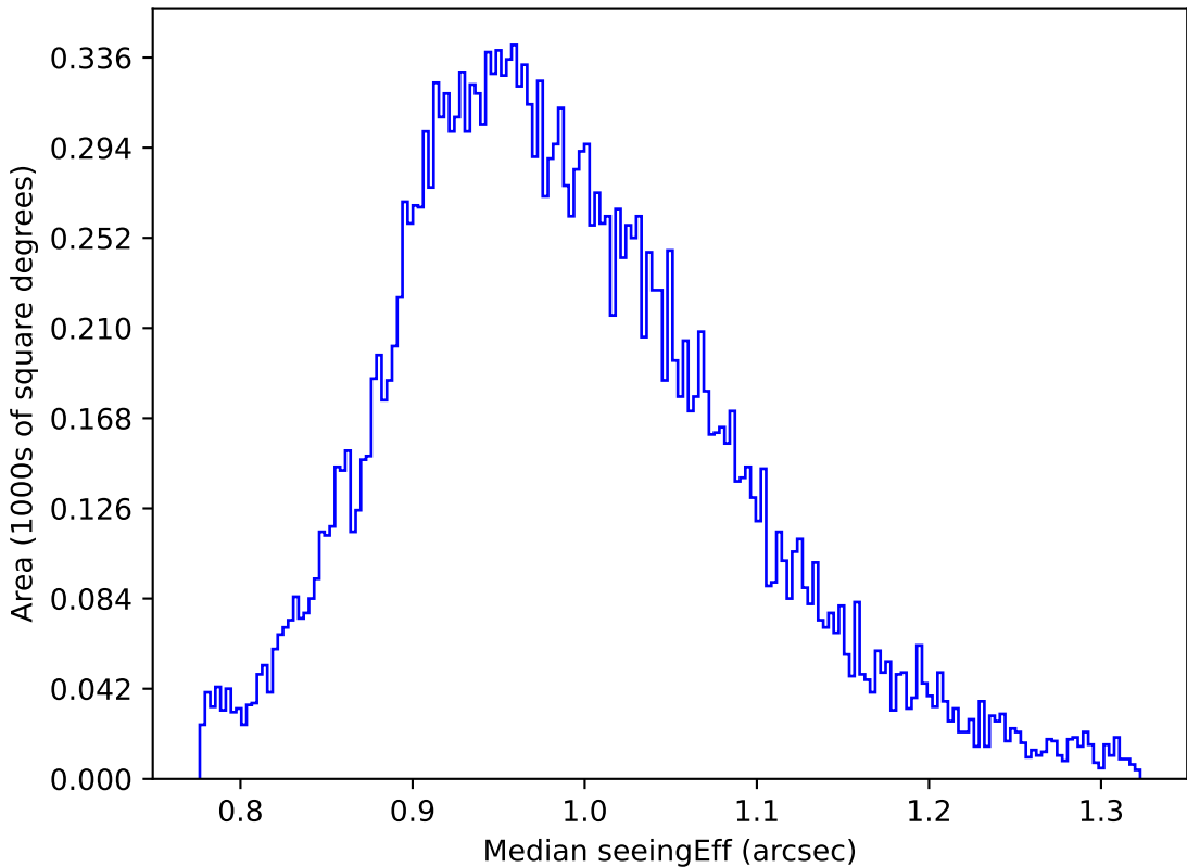
weather_cloudso14v3.4_10yrs Yr 1 y band: Median seeingEff
