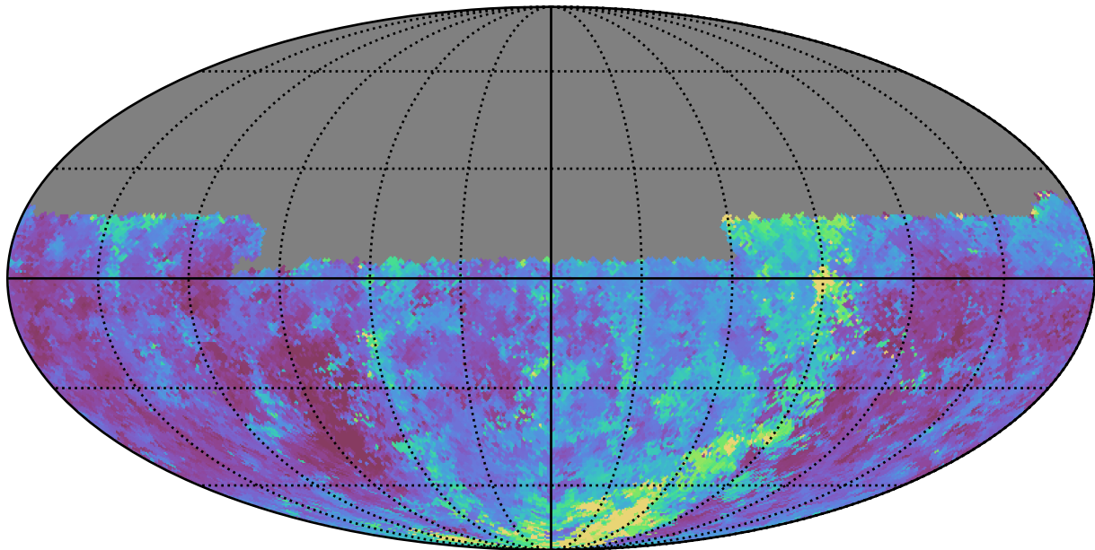
weather_cloudso14v3.4_10yrs Yr 1 u band: Median seeingEff
