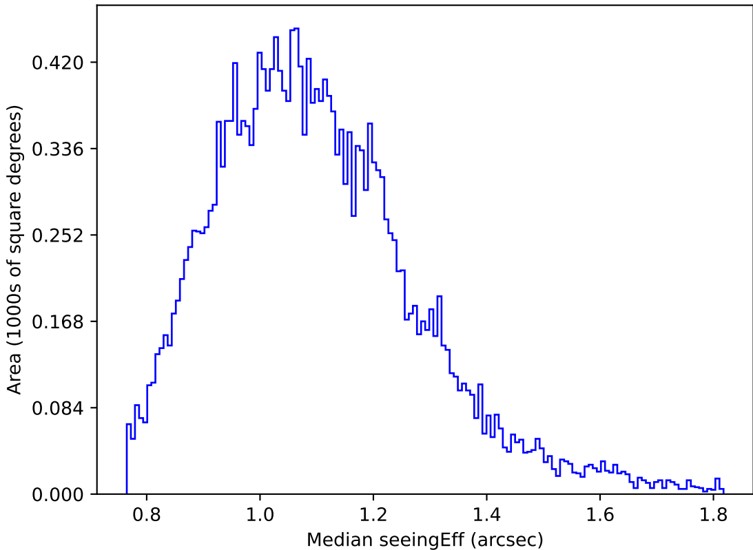
weather_cloudso14v3.4_10yrs Yr 1 u band: Median seeingEff
