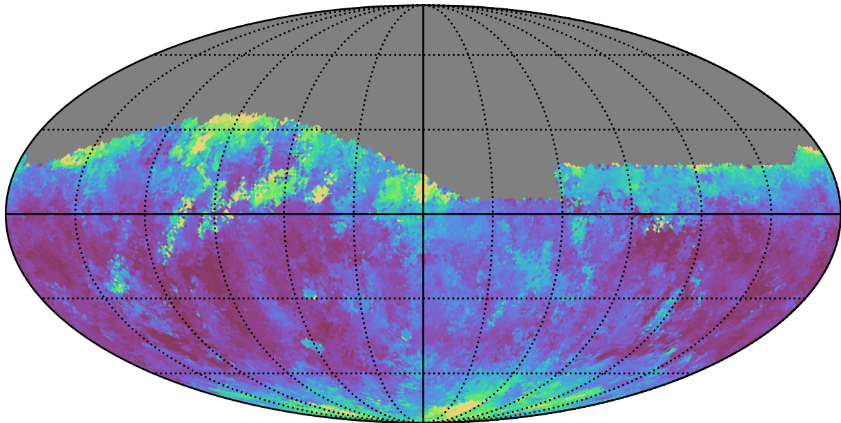
weather_cloudso14v3.4_10yrs Yr 1 r band: Median seeingEff
