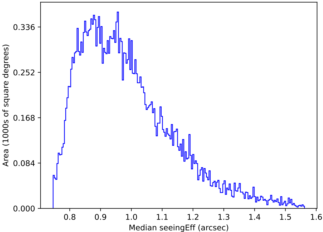
weather_cloudso14v3.4_10yrs Yr 1 r band: Median seeingEff
