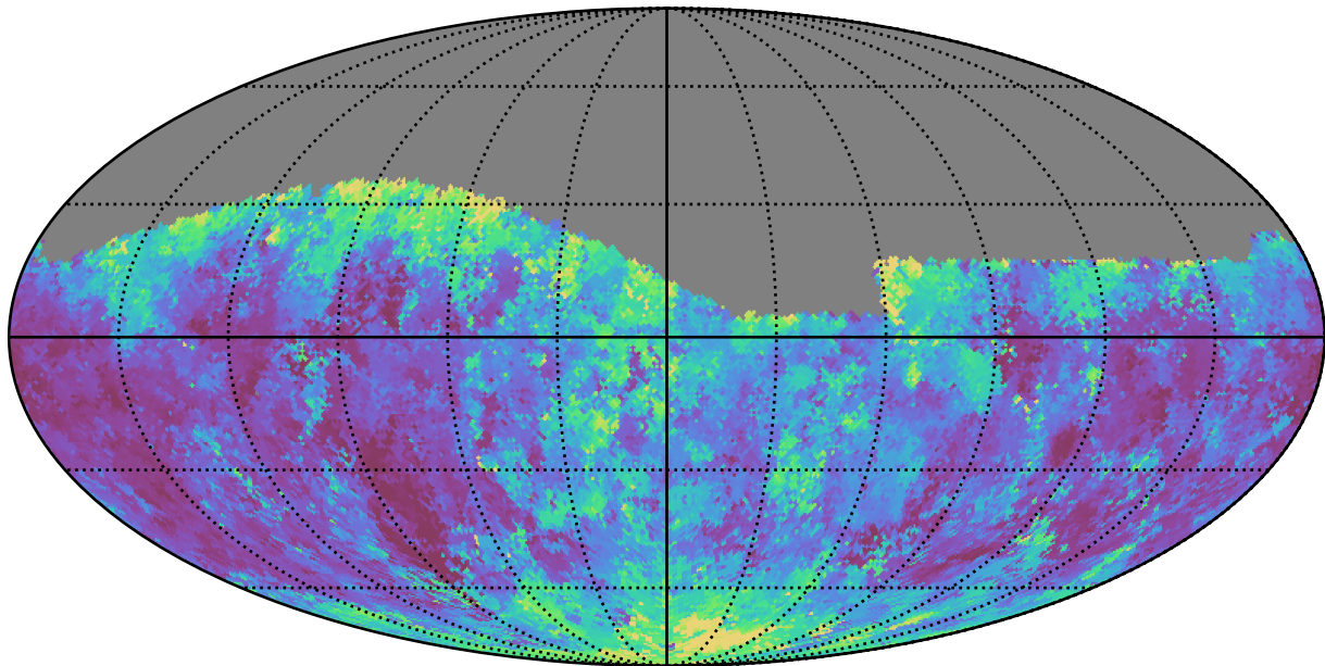
weather_cloudso14v3.4_10yrs Yr 1 g band: Median seeingEff
