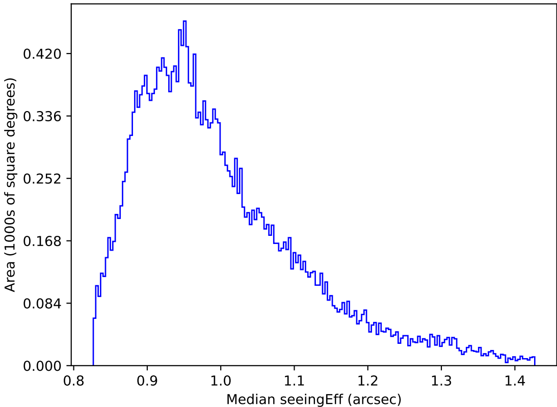
weather_cloudso14v3.4_10yrs Yr 1 all bands: Median seeingEff
