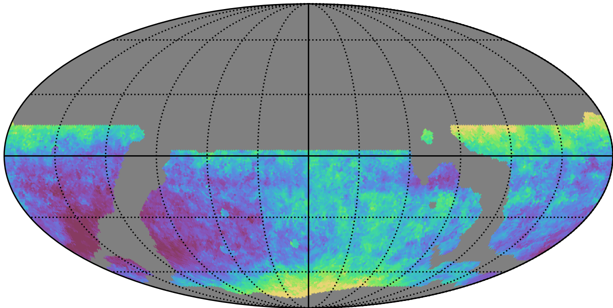
weather_cloudso14v3.4_10yrs WFD z band: Median seeingEff
