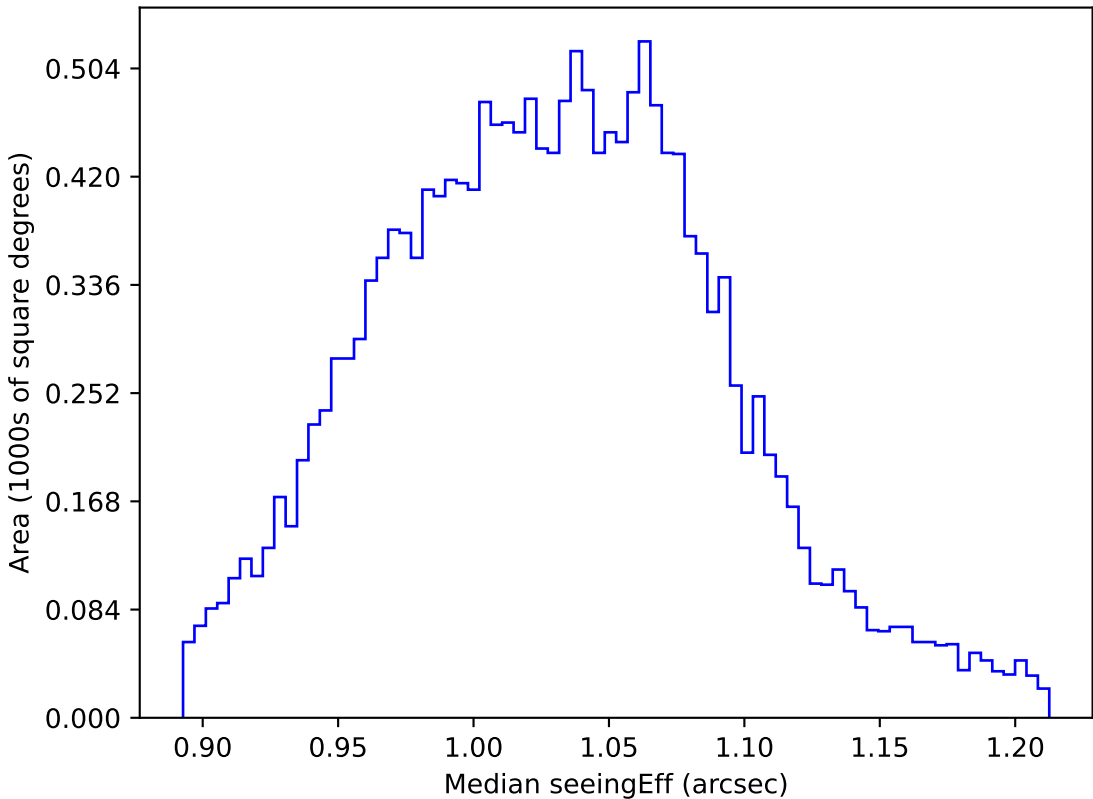
weather_cloudso14v3.4_10yrs WFD z band: Median seeingEff
