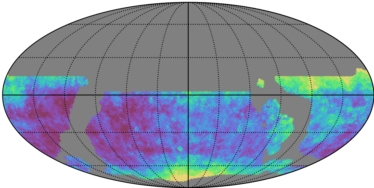
weather_cloudso14v3.4_10yrs WFD y band: Median seeingEff
