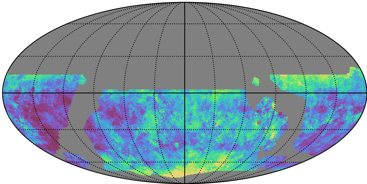
weather_cloudso14v3.4_10yrs WFD u band: Median seeingEff
