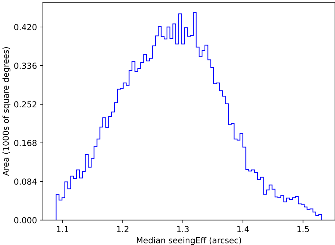
weather_cloudso14v3.4_10yrs WFD u band: Median seeingEff
