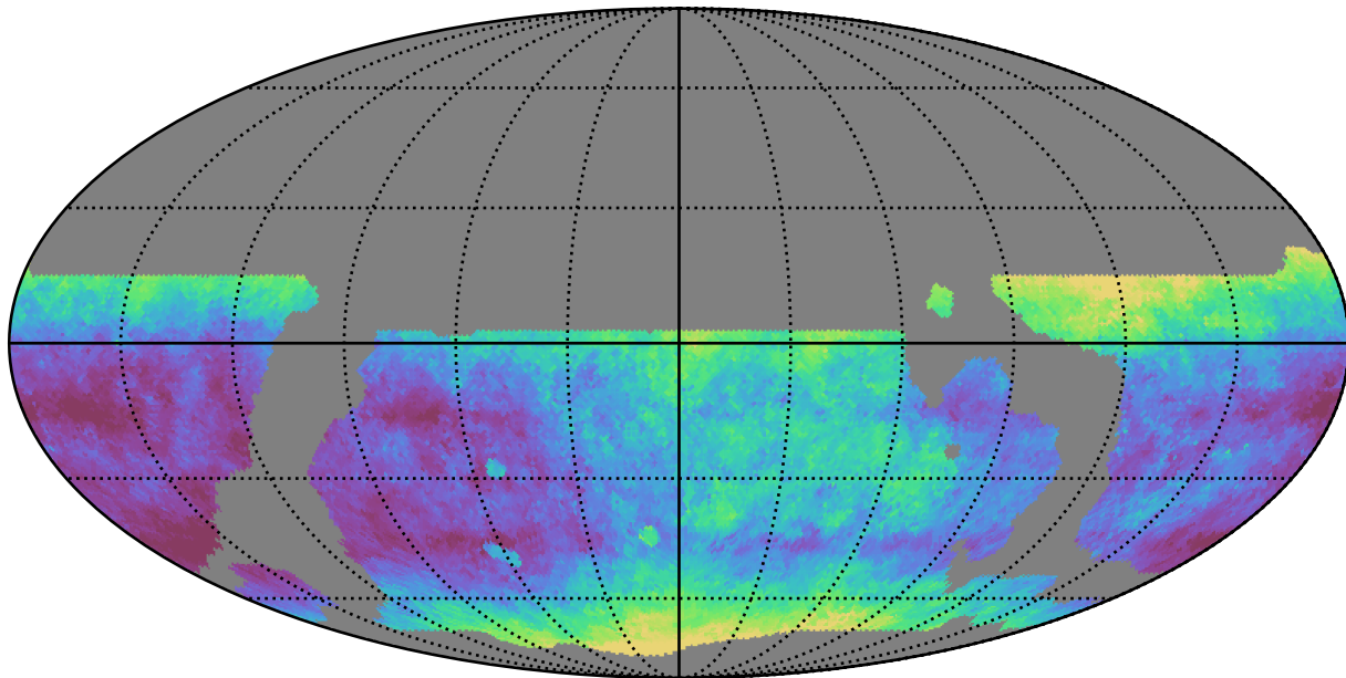
weather_cloudso14v3.4_10yrs WFD r band: Median seeingEff
