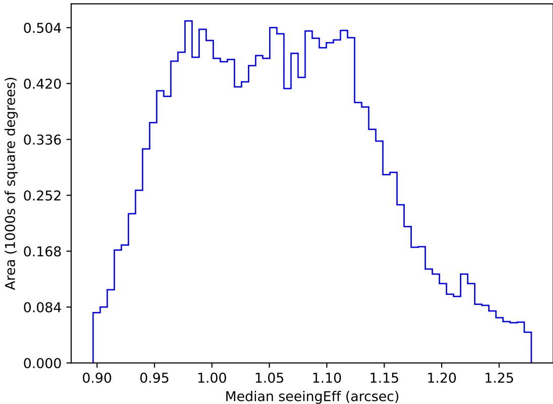
weather_cloudso14v3.4_10yrs WFD r band: Median seeingEff
