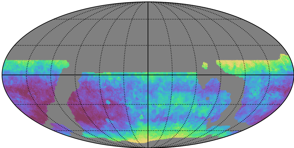
weather_cloudso14v3.4_10yrs WFD i band: Median seeingEff
